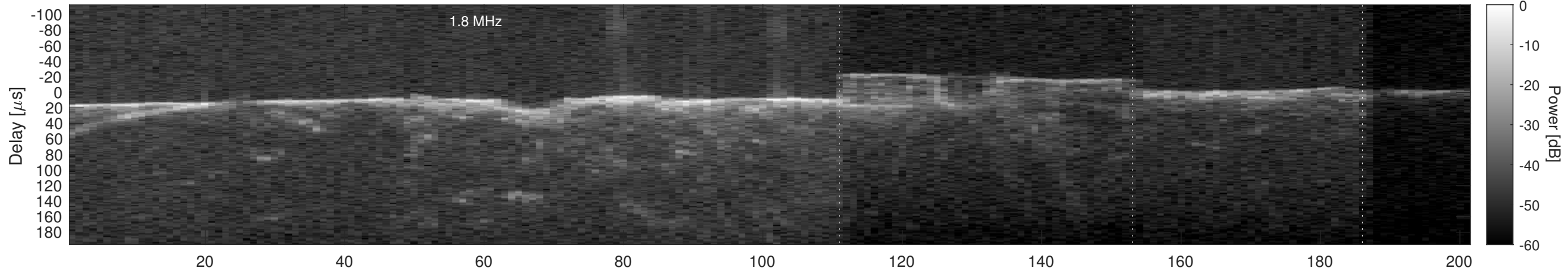
Orbit 2704, Cluttergram
