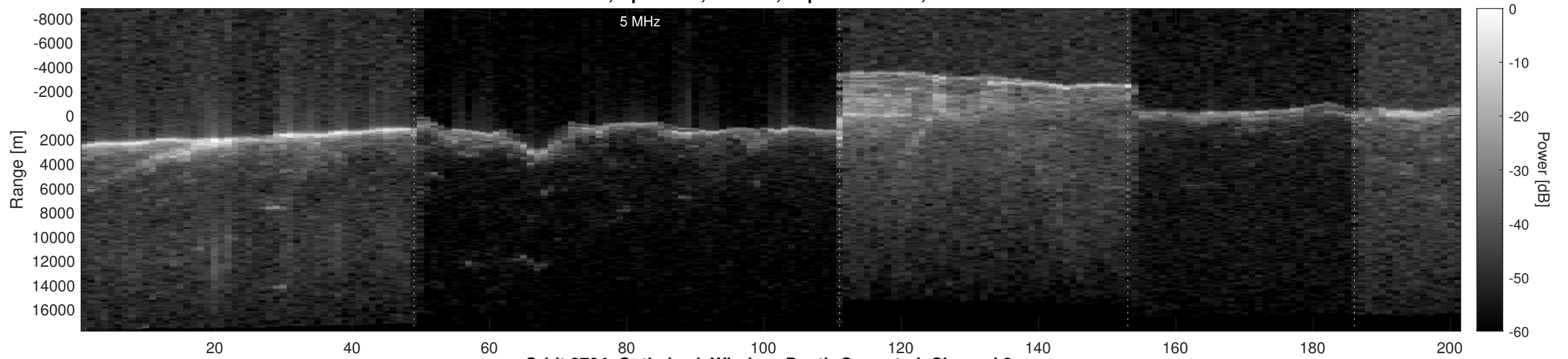
Orbit 2704, Optimized, Window, Depth-Corrected, Channel 2
