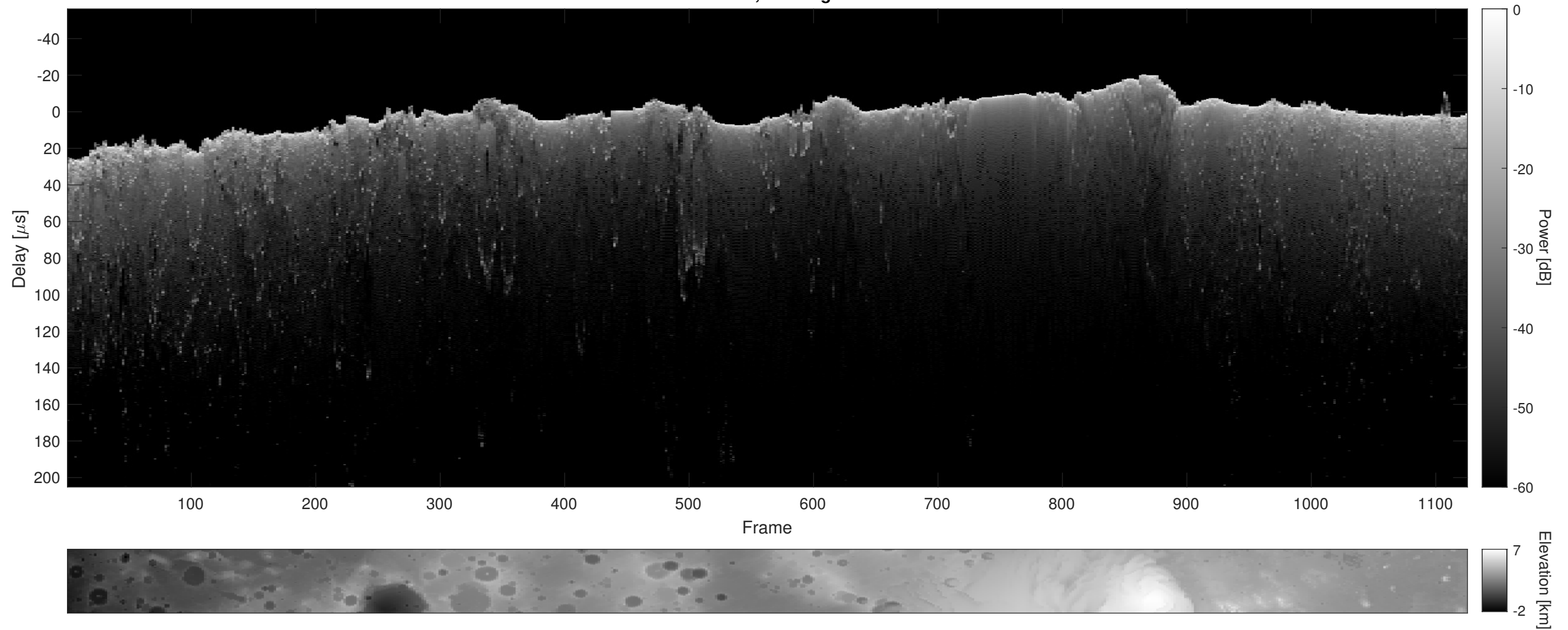
Orbit 2705, Cluttergram
