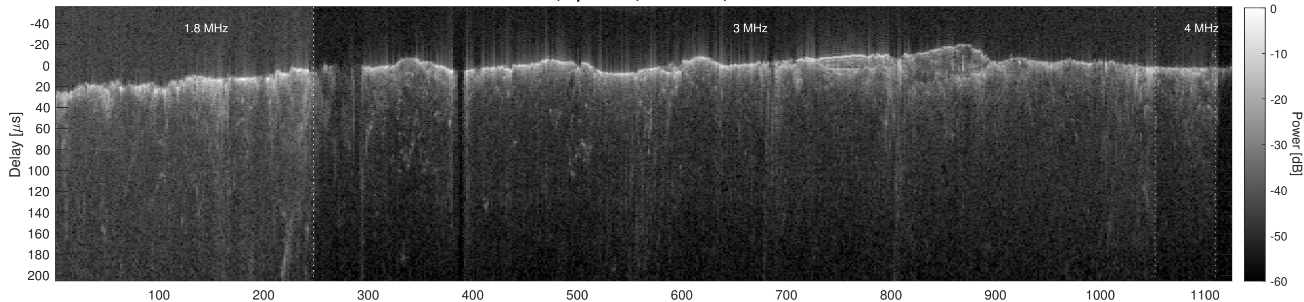
Orbit 2705, Cluttergram
