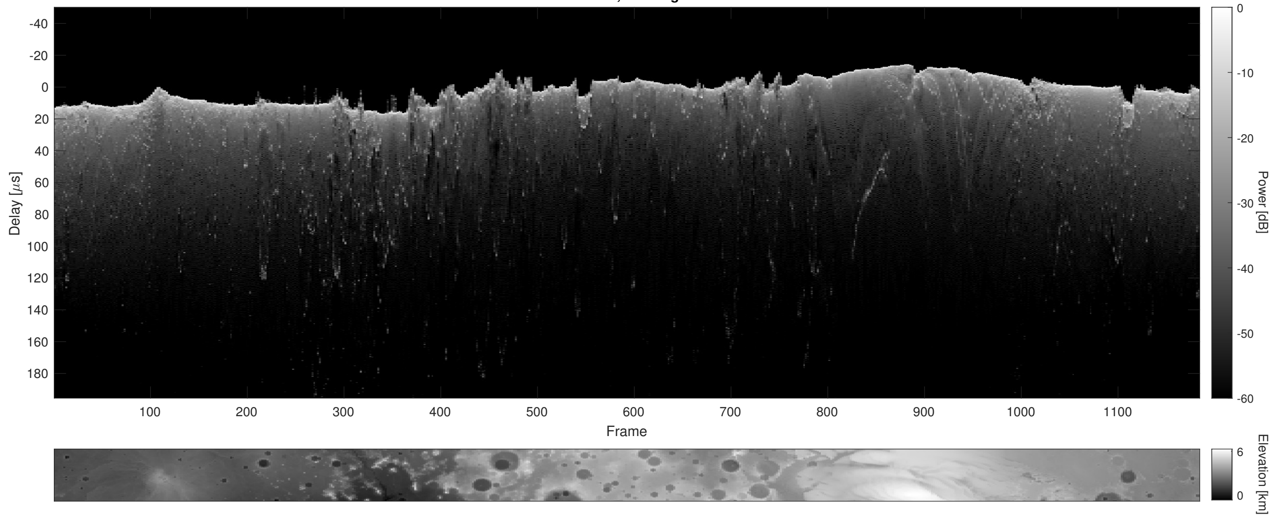
Orbit 2706, Cluttergram
