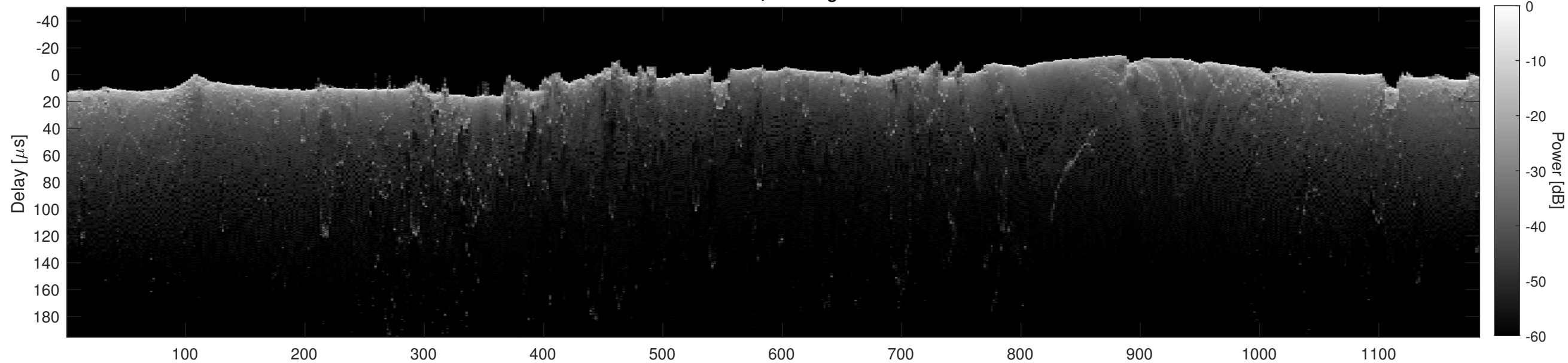
Orbit 2706, Cluttergram
