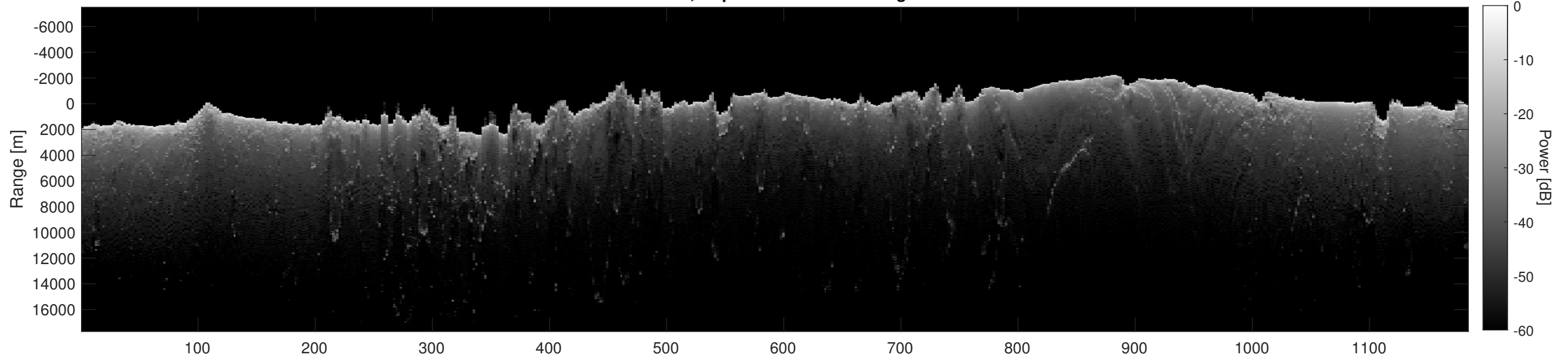
Orbit 2706, Depth-Corrected Cluttergram
