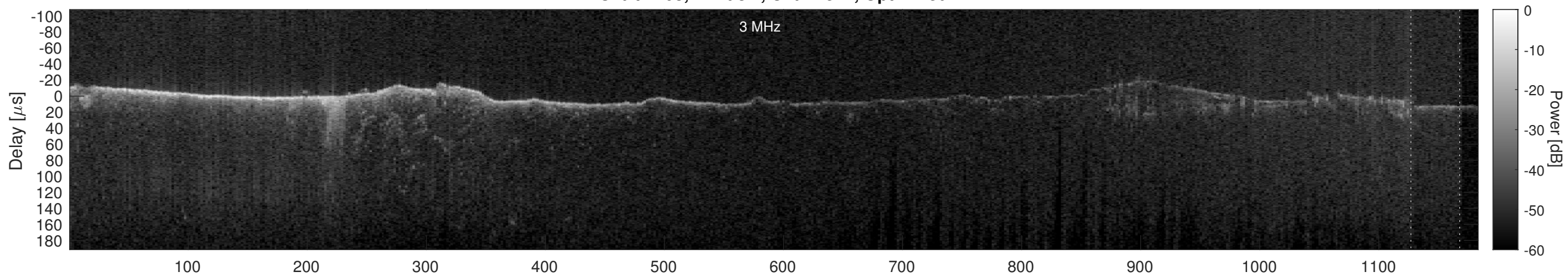
Orbit 2708, Cluttergram
