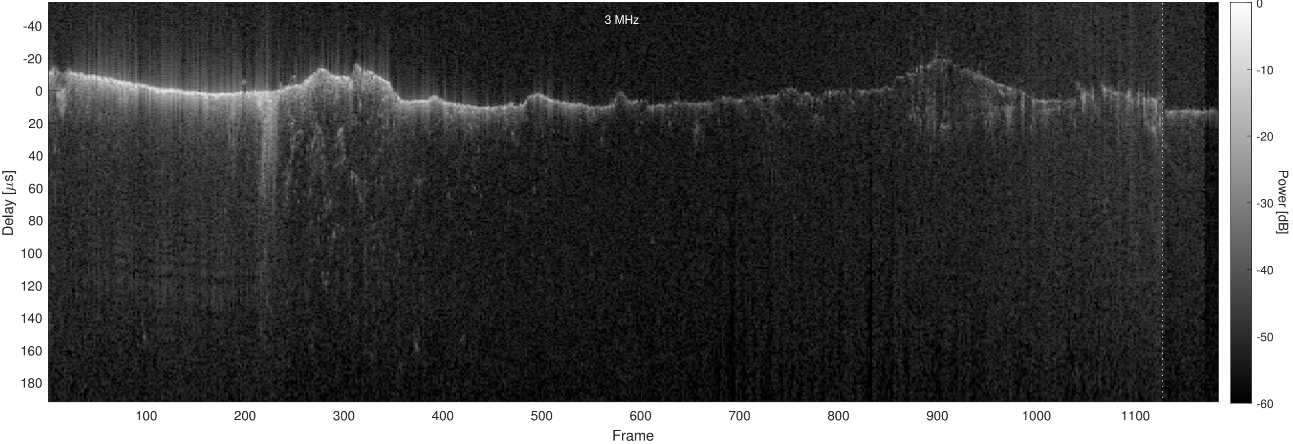
Orbit 2708, Optimized, No Window, Channel 2
