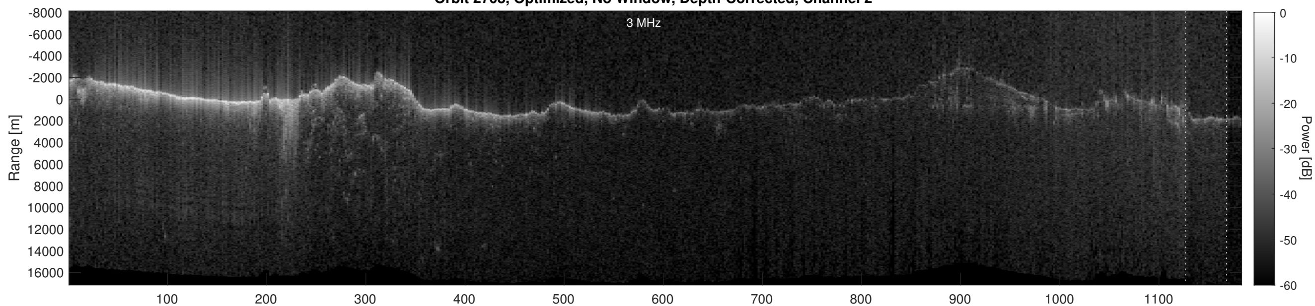
Orbit 2708, Depth-Corrected Cluttergram
