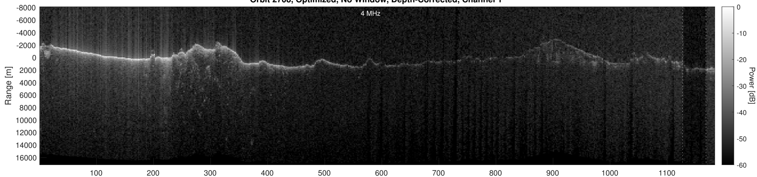
Orbit 2708, Optimized, No Window, Depth-Corrected, Channel 2
