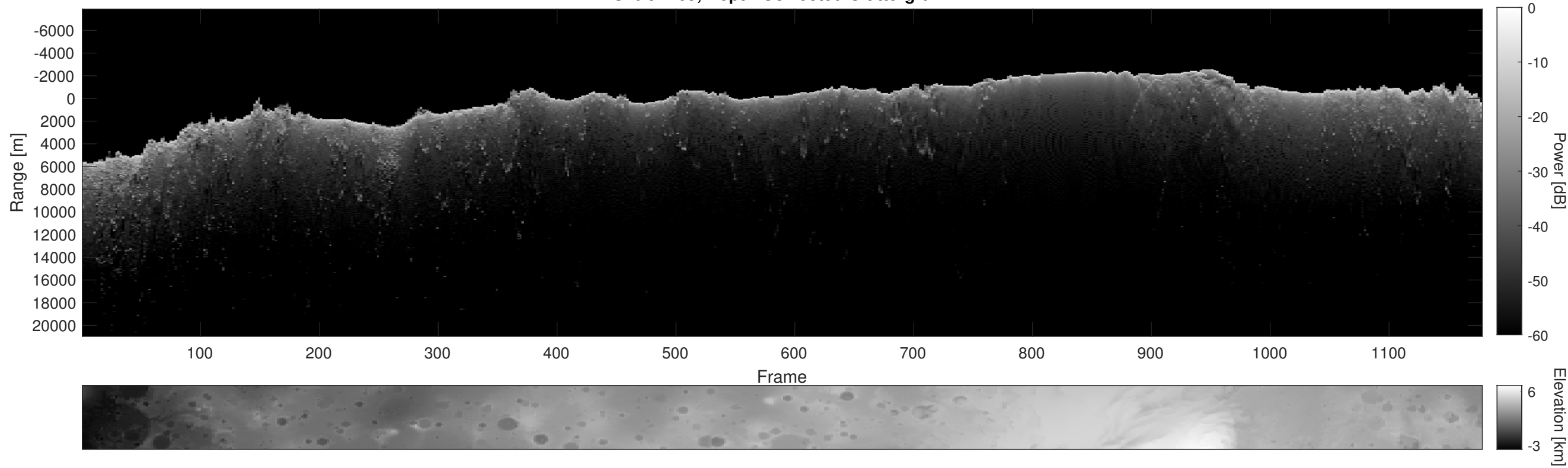
Orbit 2709, Depth-Corrected Cluttergram
