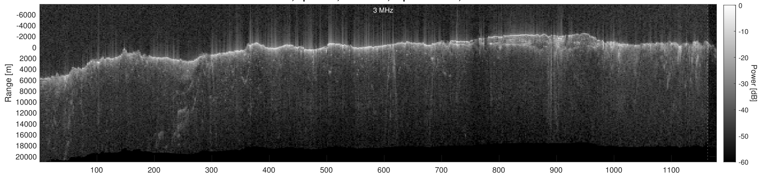
Orbit 2709, Depth-Corrected Cluttergram
