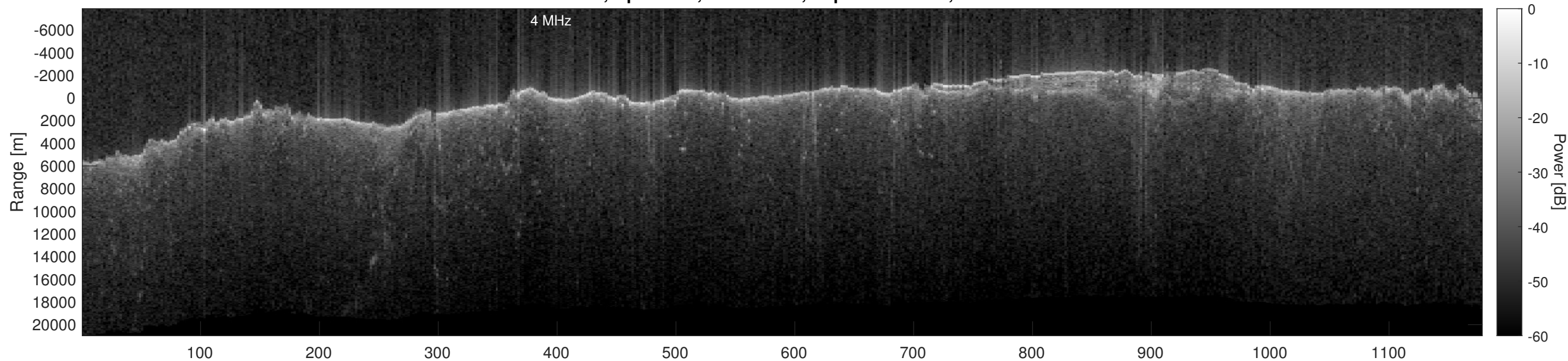
Orbit 2709, Optimized, No Window, Depth-Corrected, Channel 2
