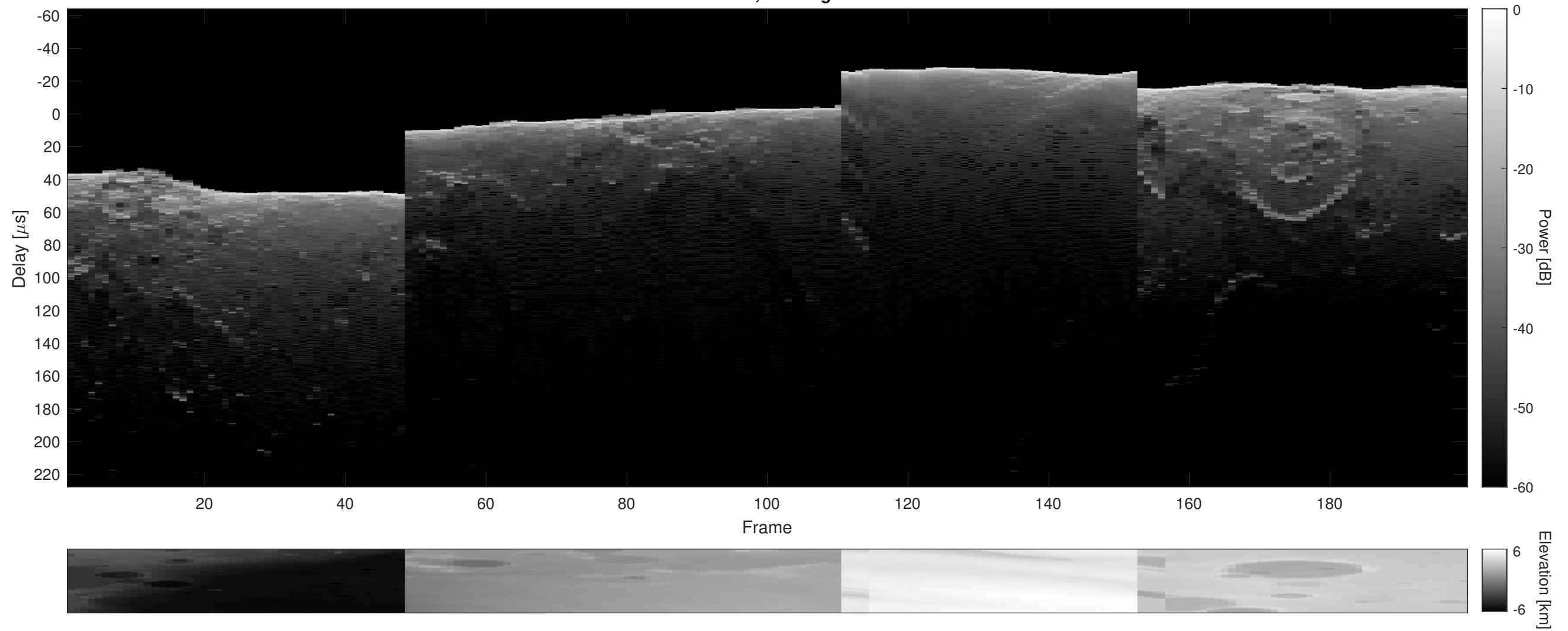
Orbit 2710, Cluttergram
