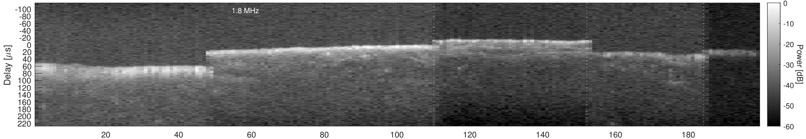
Orbit 2710, Window, Channel 2, Chapman
