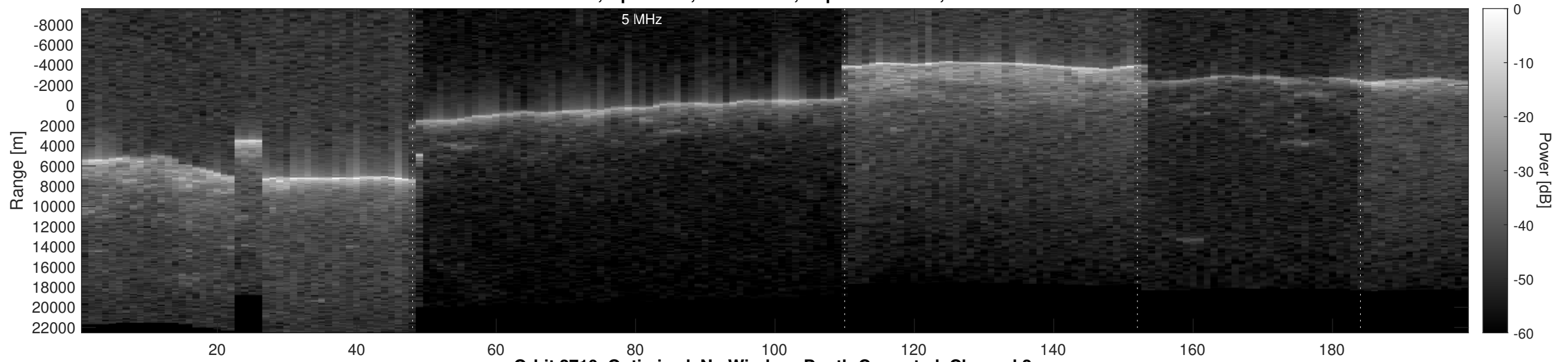
Orbit 2710, Optimized, No Window, Depth-Corrected, Channel 2
