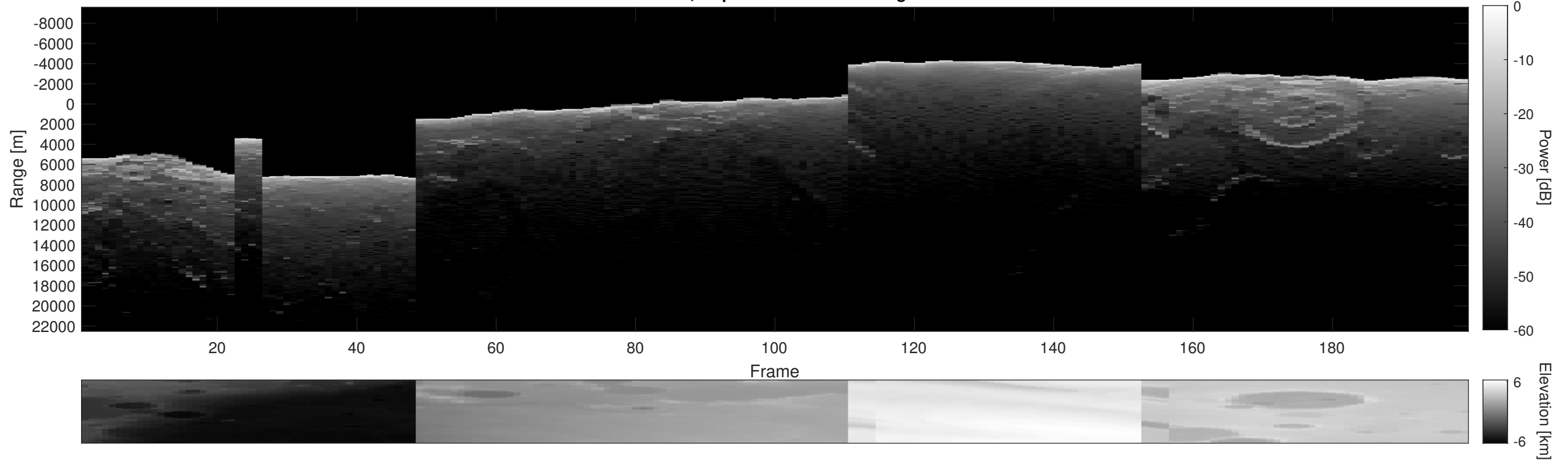
Orbit 2710, Depth-Corrected Cluttergram
