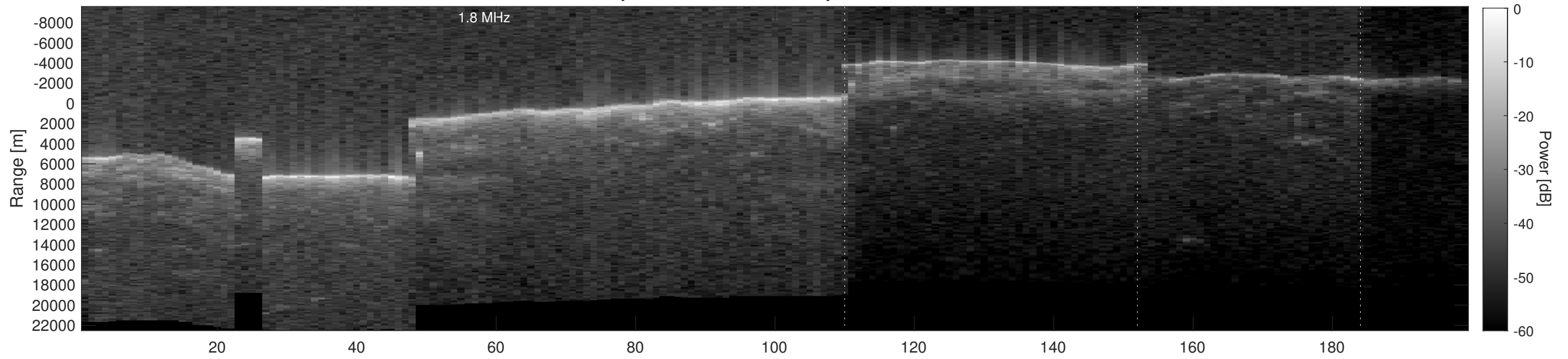
Orbit 2710, Depth-Corrected Cluttergram
