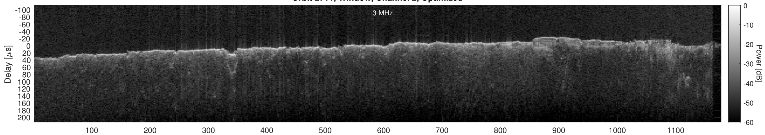
Orbit 2711, Cluttergram
