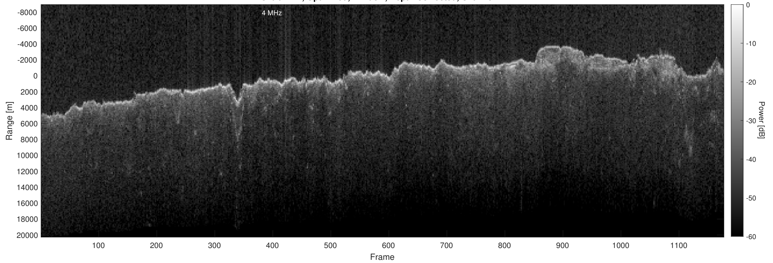
Orbit 2711, Optimized, Window, Depth-Corrected, Channel 2
