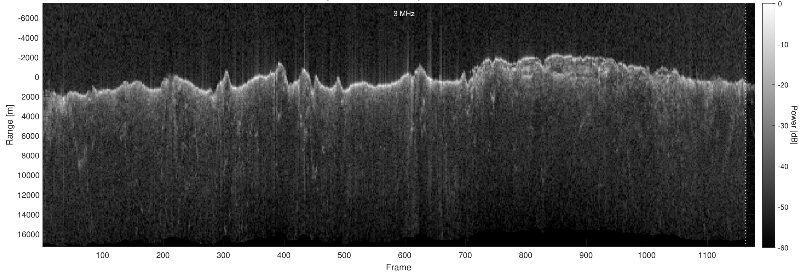
Orbit 2713, Optimized, Window, Depth-Corrected, Channel 2
