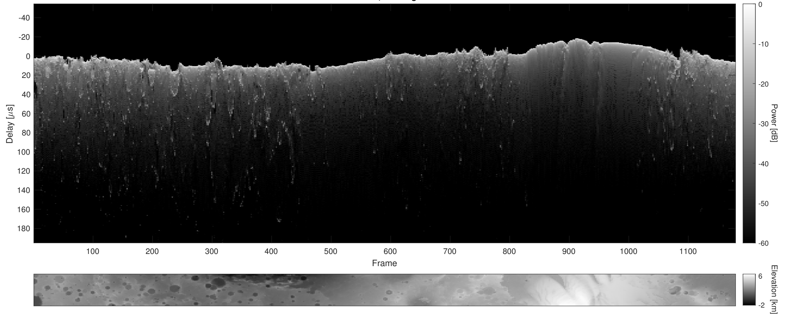
Orbit 2714, Cluttergram
