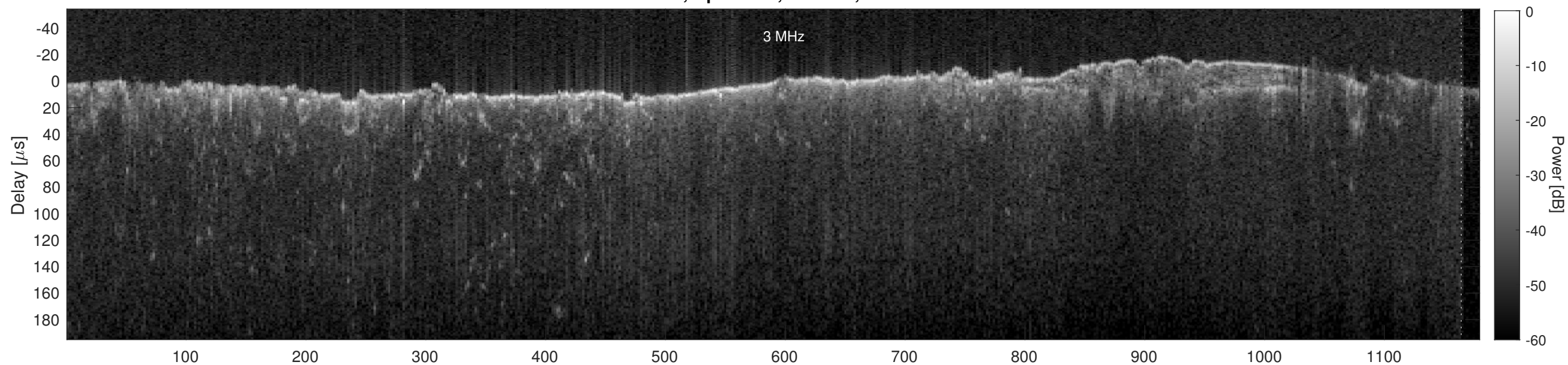
Orbit 2714, Cluttergram
