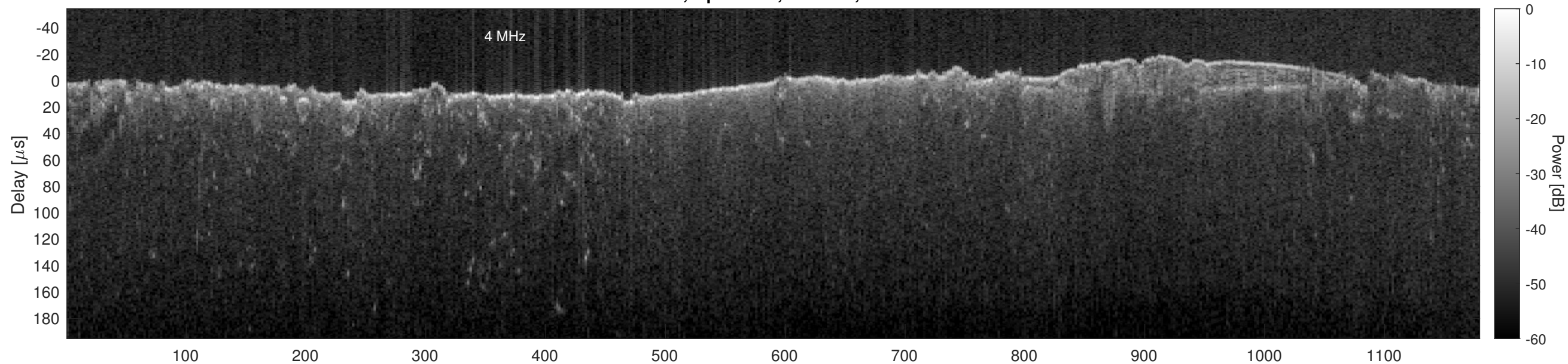
Orbit 2714, Optimized, Window, Channel 2
