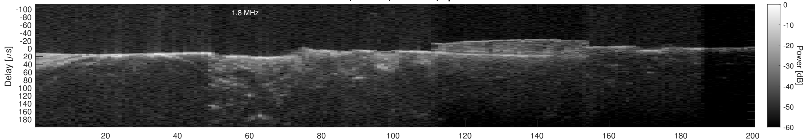
Orbit 2715, Cluttergram
