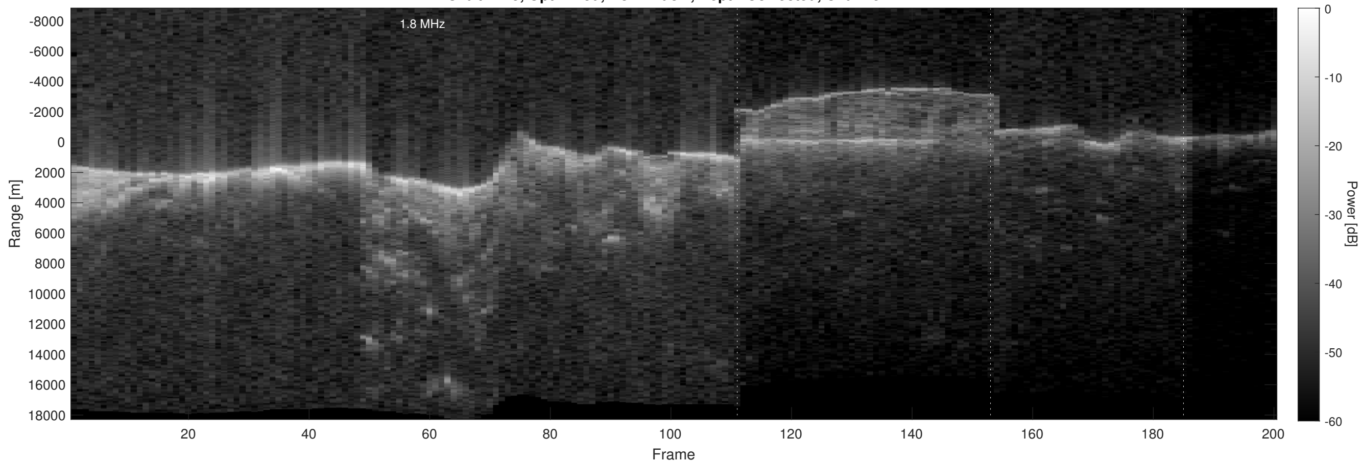
Orbit 2715, Optimized, No Window, Depth-Corrected, Channel 2
