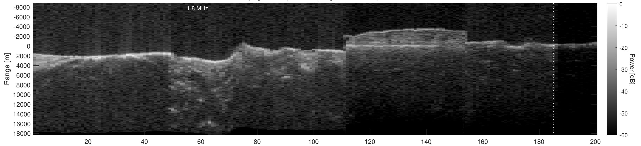
Orbit 2715, Depth-Corrected Cluttergram
