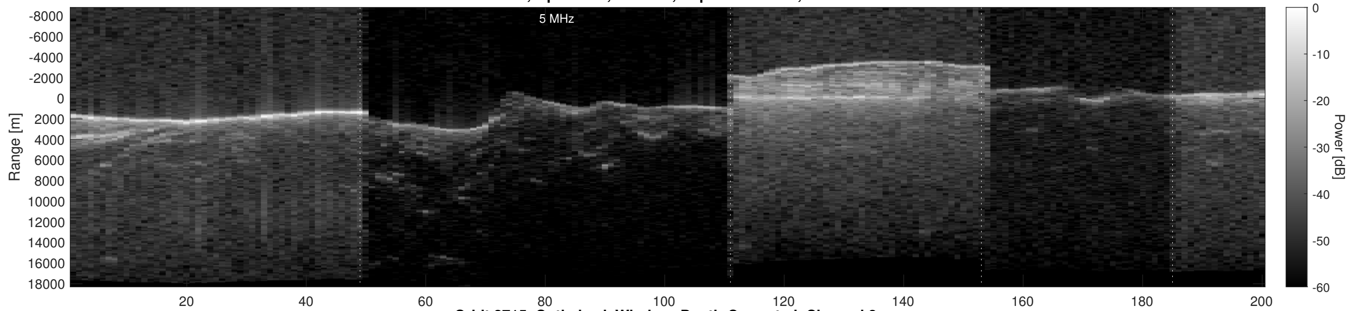
Orbit 2715, Optimized, Window, Depth-Corrected, Channel 2
