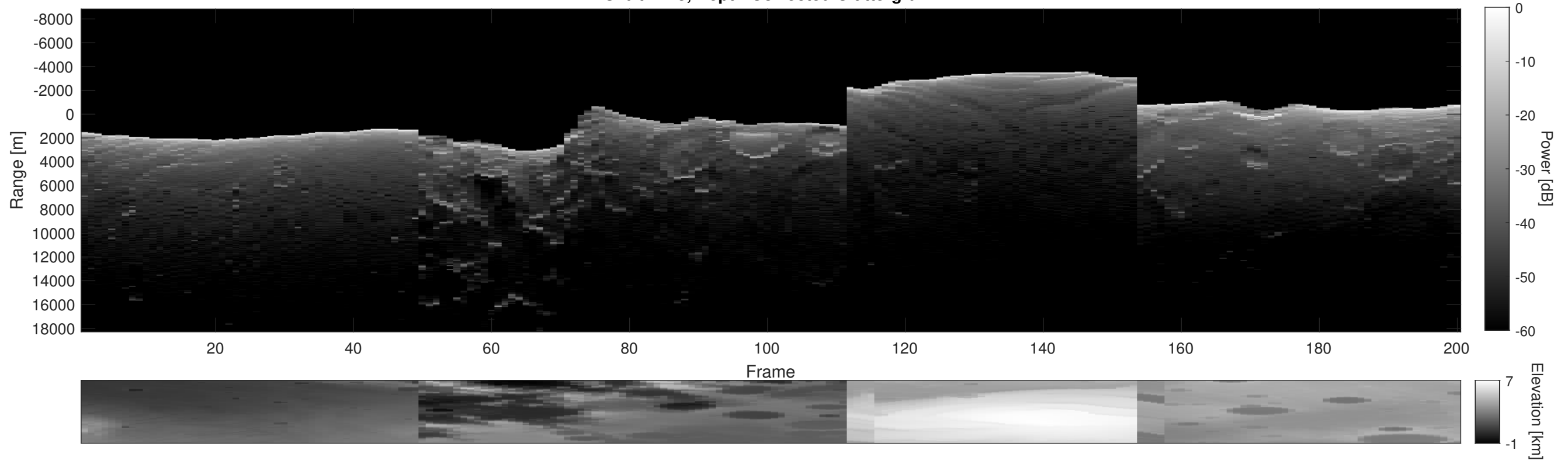
Orbit 2715, Depth-Corrected Cluttergram
