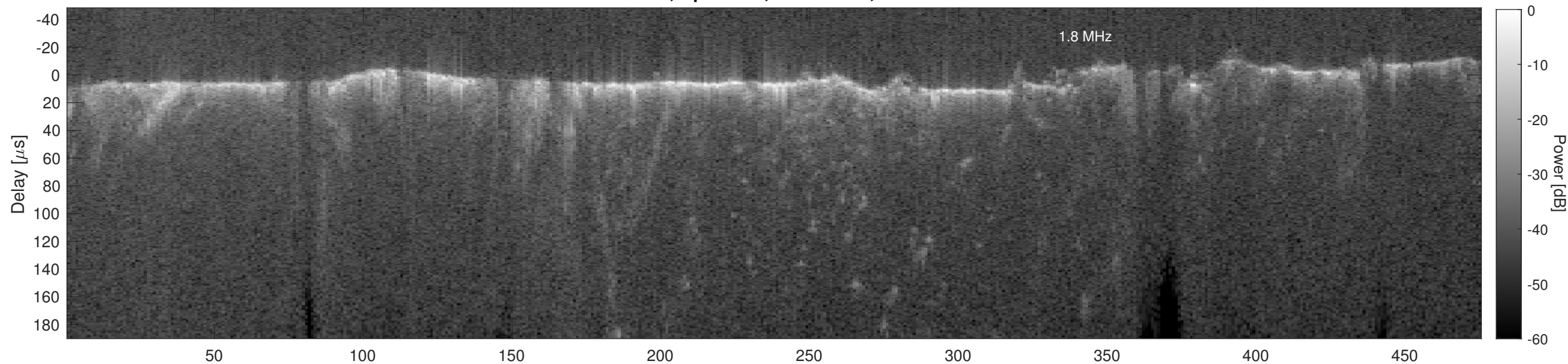
Orbit 2717, Cluttergram
