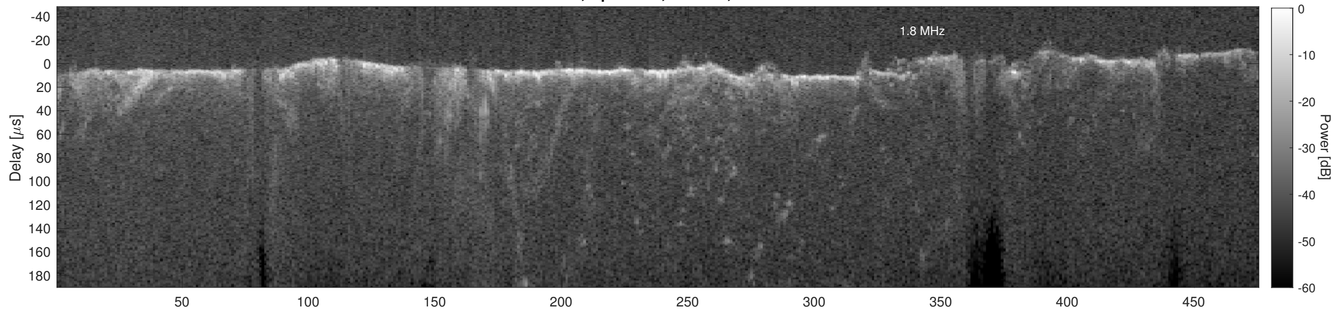
Orbit 2717, Cluttergram
