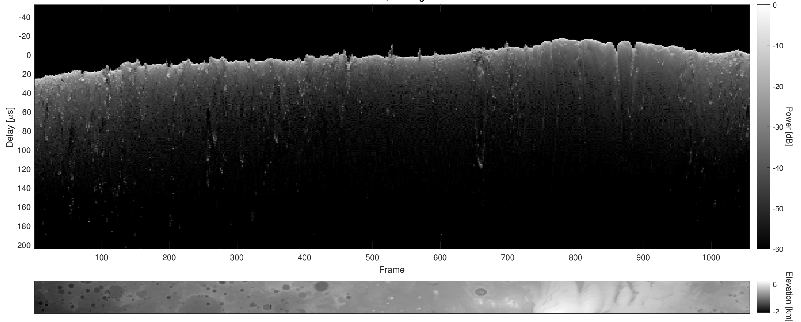
Orbit 2718, Cluttergram
