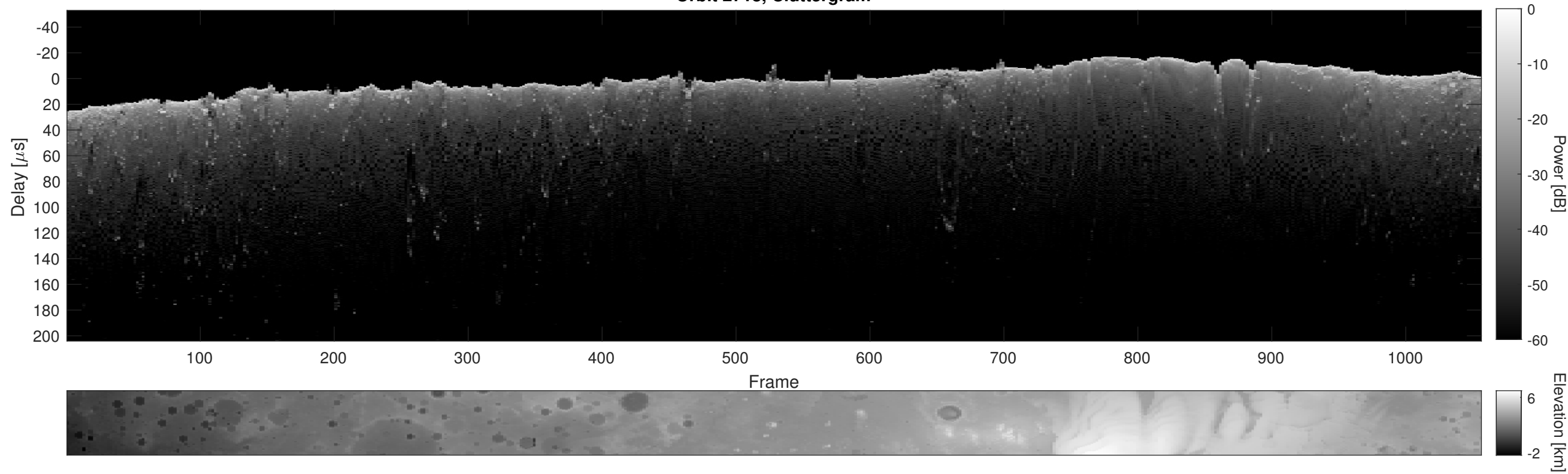
Orbit 2718, Cluttergram
