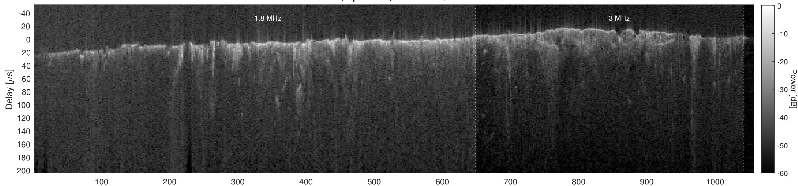
Orbit 2718, Cluttergram
