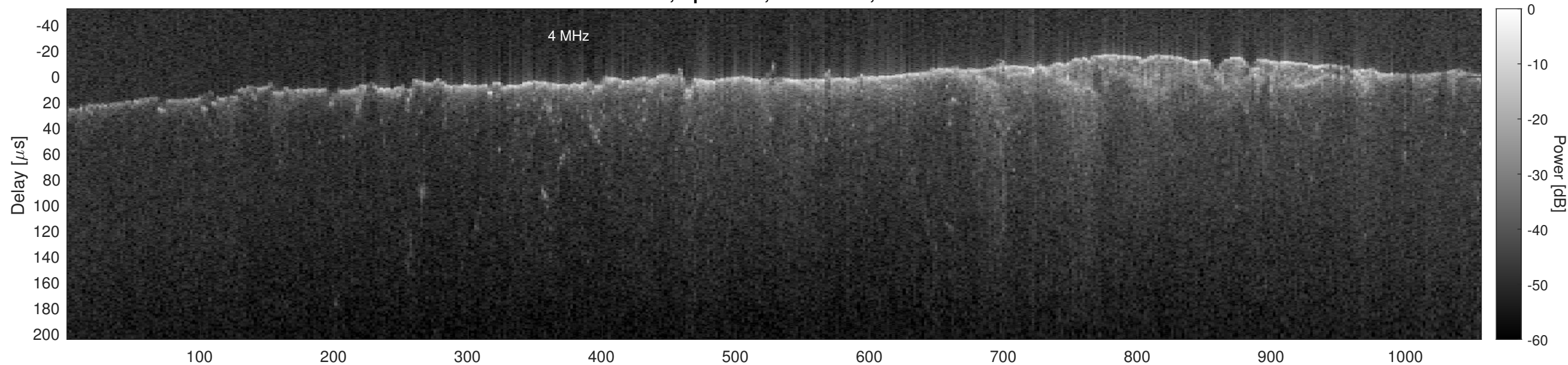
Orbit 2718, Optimized, No Window, Channel 2
