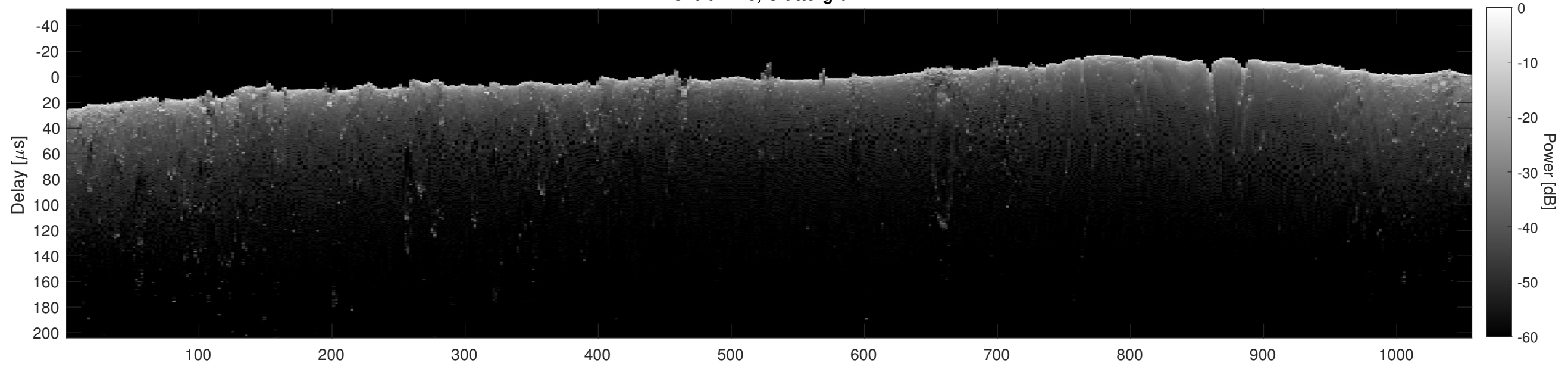
Orbit 2718, Cluttergram
