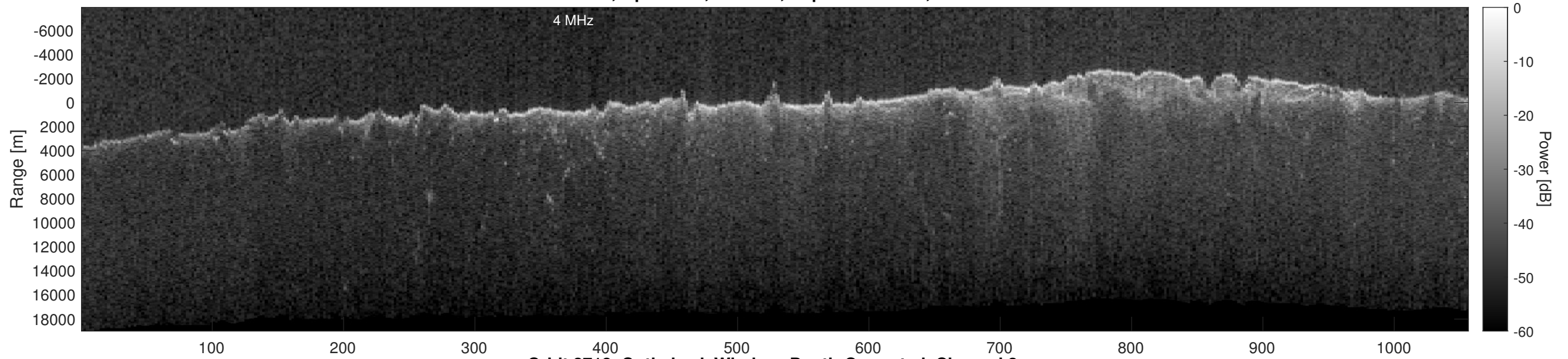
Orbit 2718, Optimized, Window, Depth-Corrected, Channel 2
