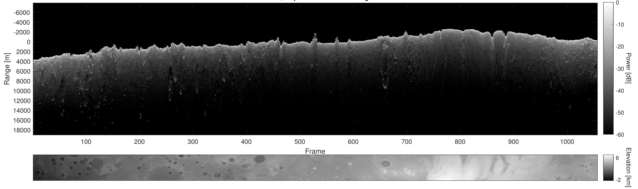
Orbit 2718, Depth-Corrected Cluttergram
