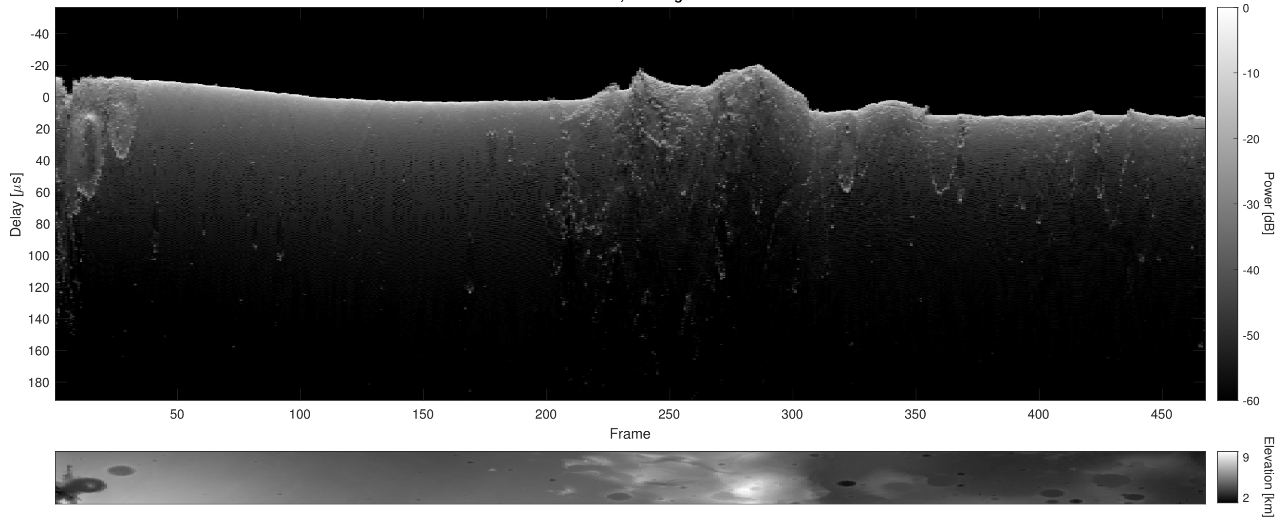
Orbit 2719, Cluttergram
