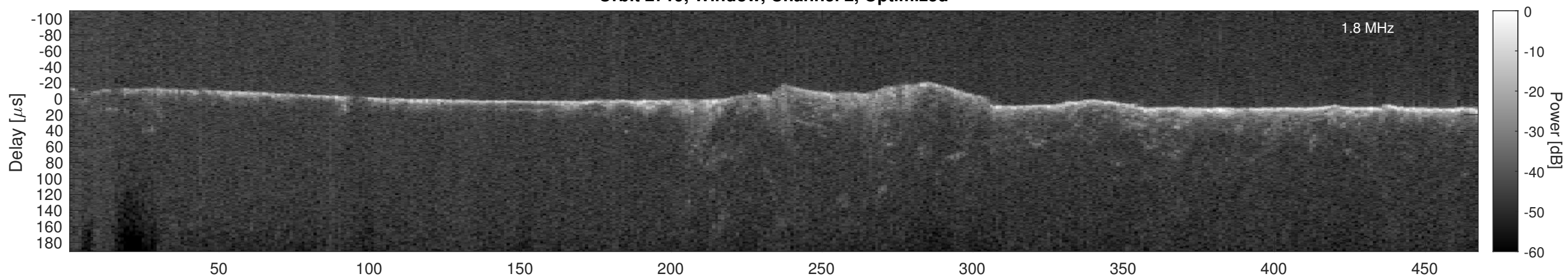
Orbit 2719, Cluttergram
