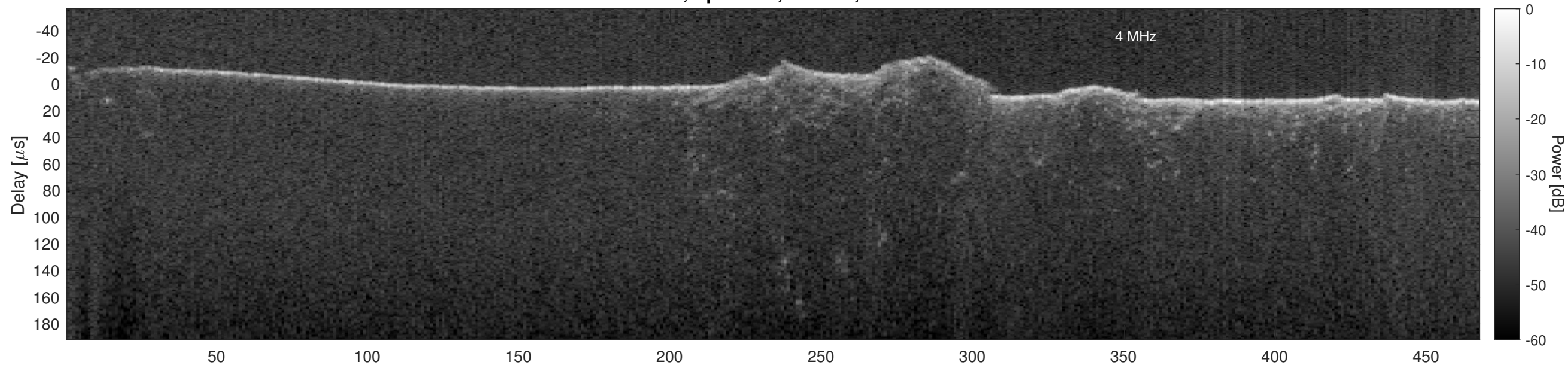
Orbit 2719, Optimized, Window, Channel 2
