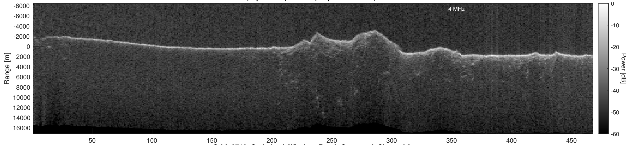
Orbit 2719, Optimized, Window, Depth-Corrected, Channel 2
