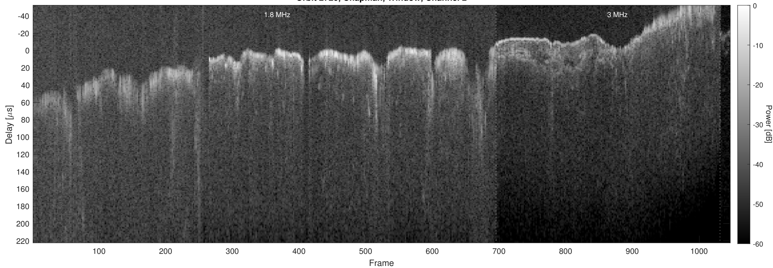
Orbit 2720, Chapman, Window, Channel 2
