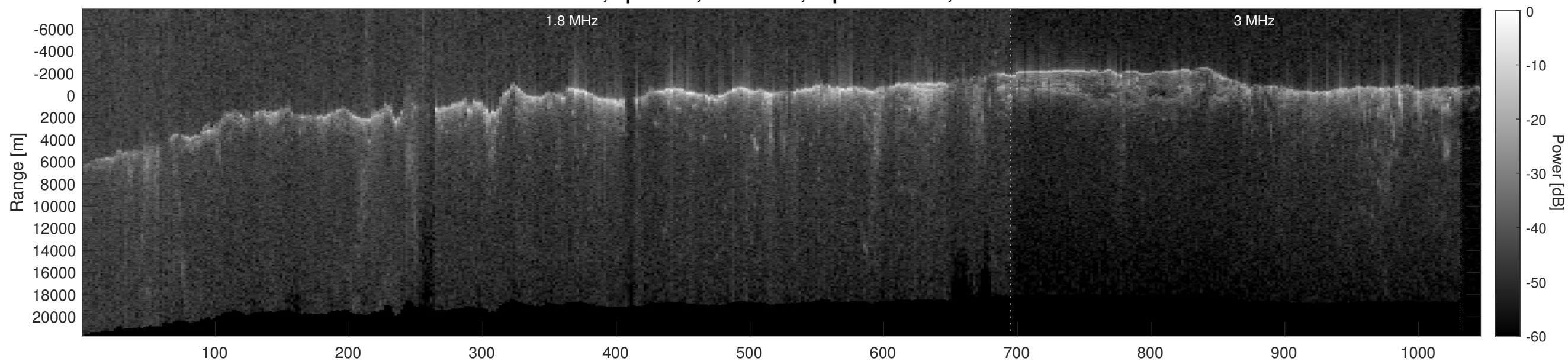
Orbit 2720, Depth-Corrected Cluttergram
