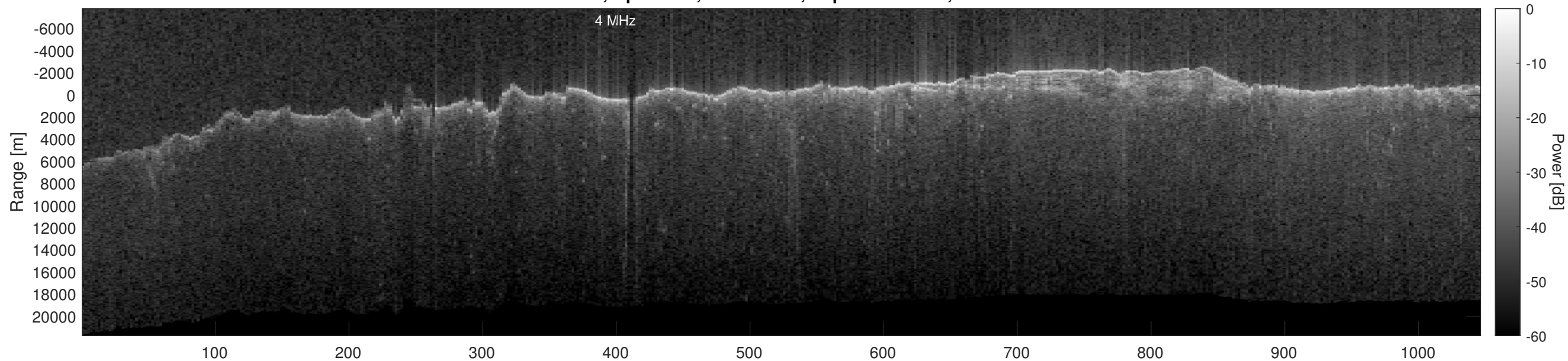
Orbit 2720, Optimized, No Window, Depth-Corrected, Channel 2
