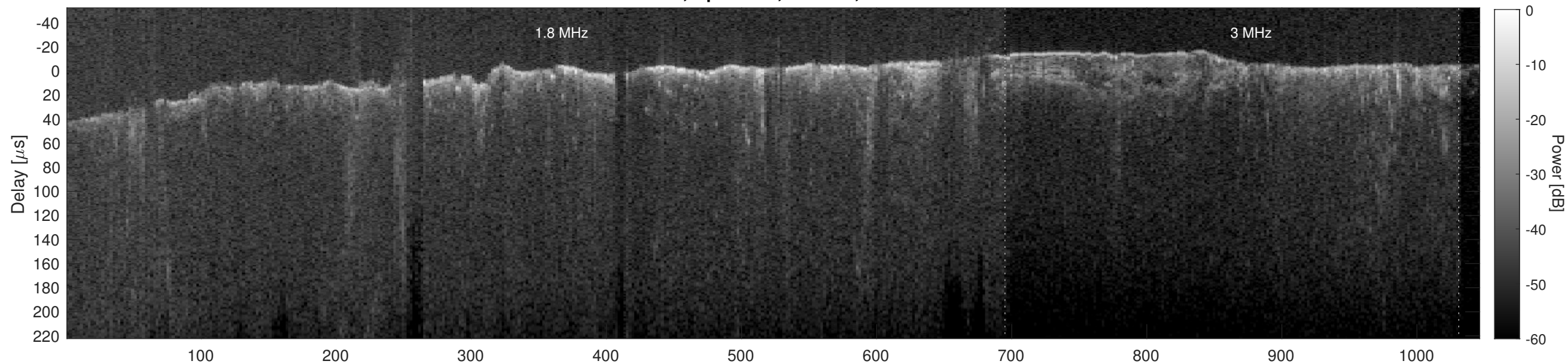
Orbit 2720, Cluttergram
