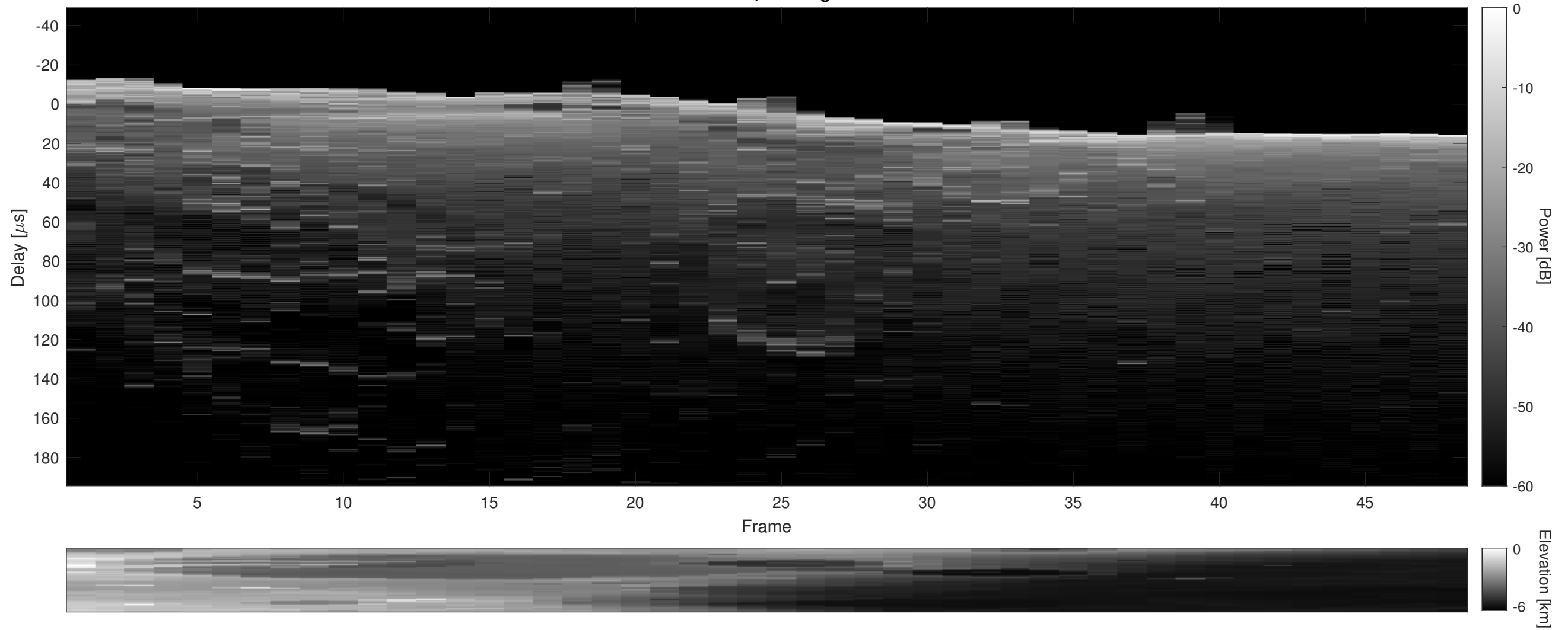
Orbit 2721, Cluttergram
