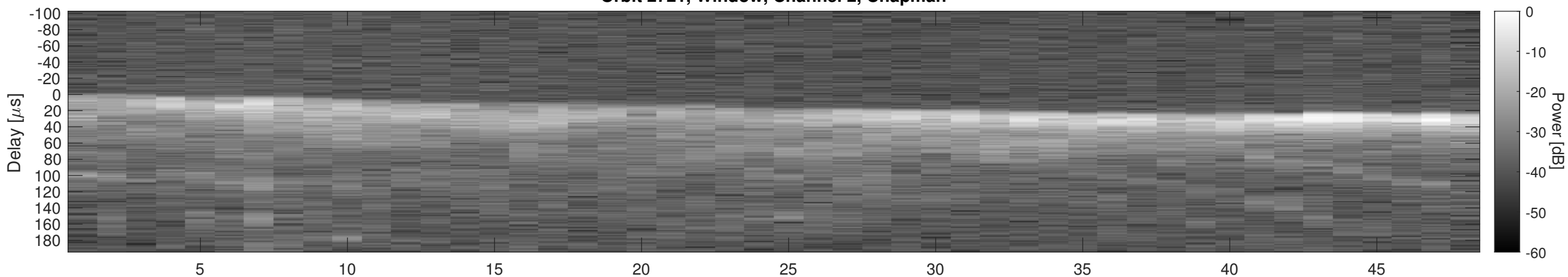
Orbit 2721, Window, Channel 2, Optimized
