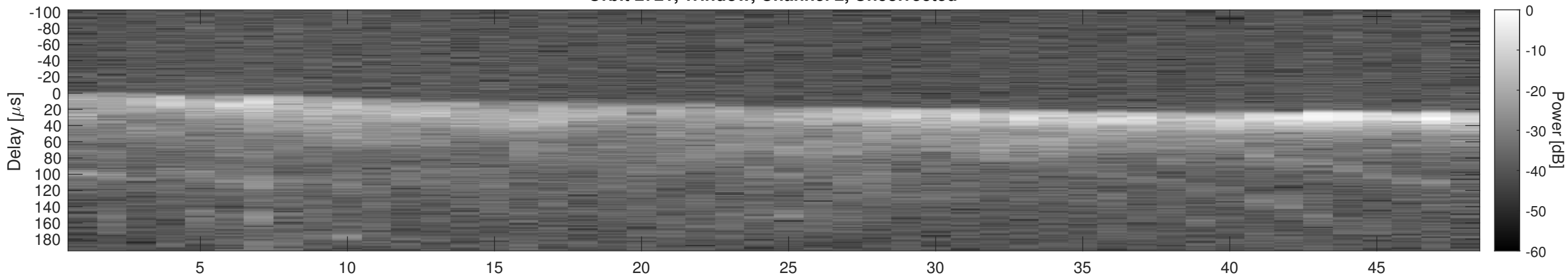
Orbit 2721, Window, Channel 2, Chapman
