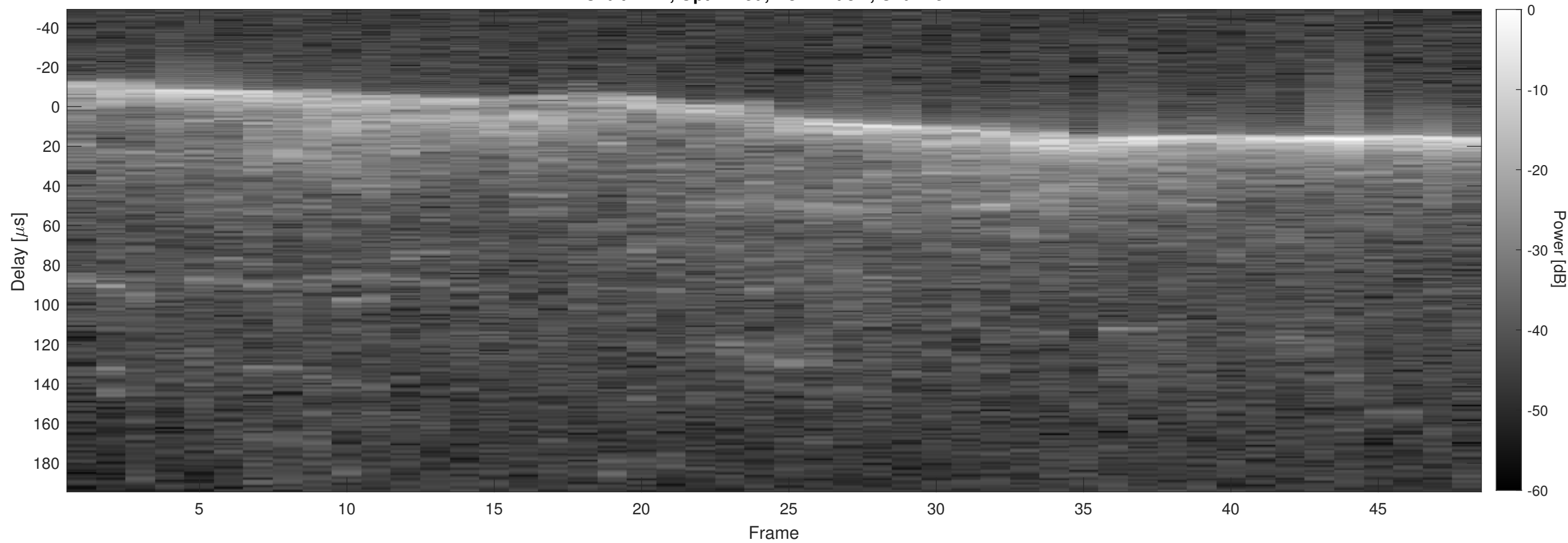
Orbit 2721, Optimized, No Window, Channel 2
