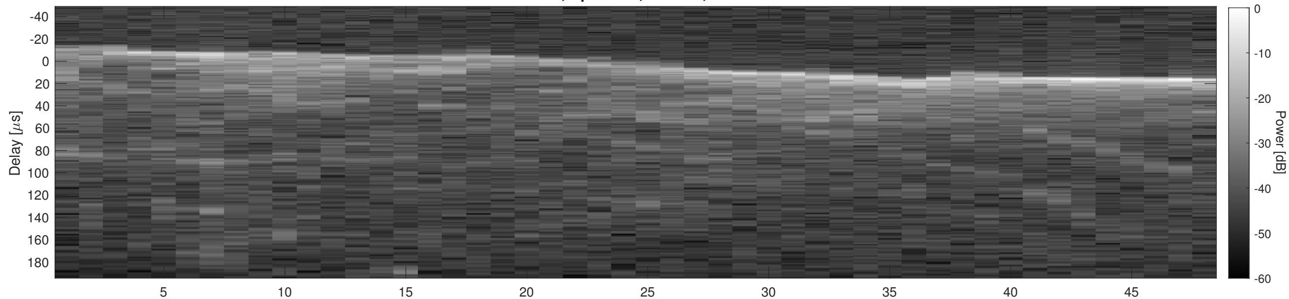
Orbit 2721, Cluttergram
