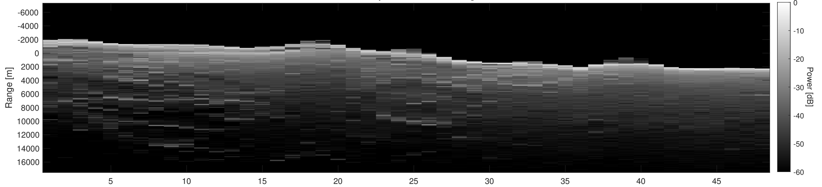
Orbit 2721, Depth-Corrected Cluttergram
