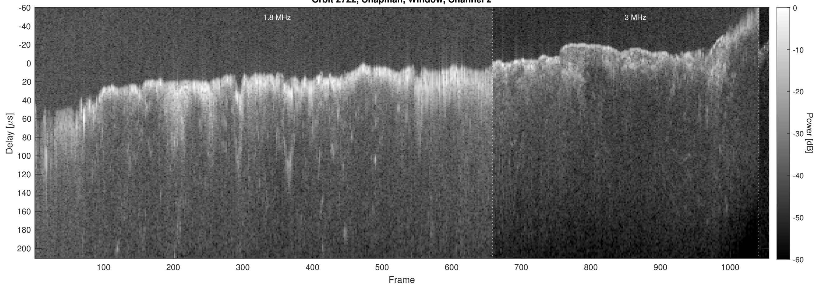
Orbit 2722, Chapman, Window, Channel 2
