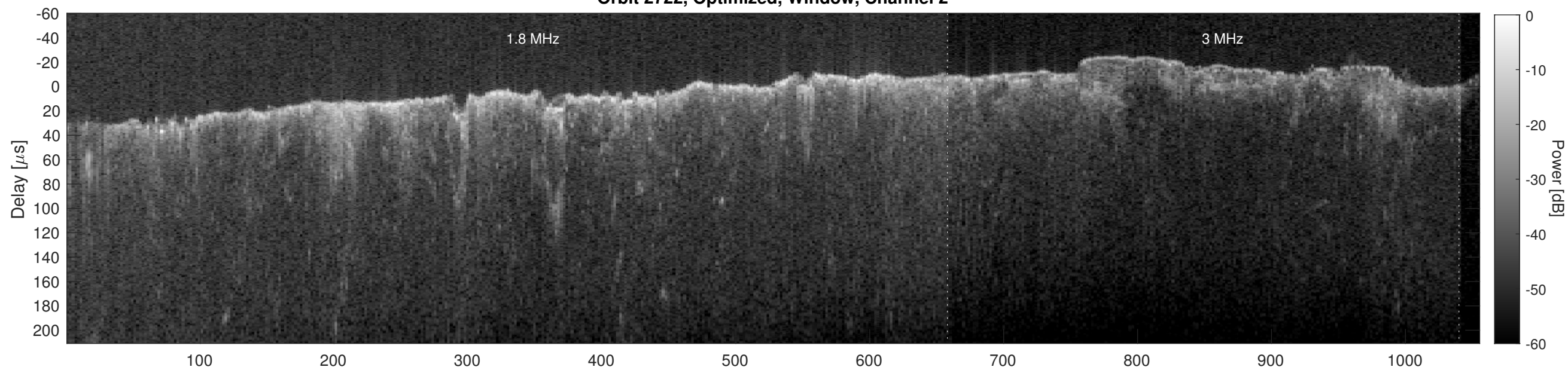
Orbit 2722, Cluttergram
