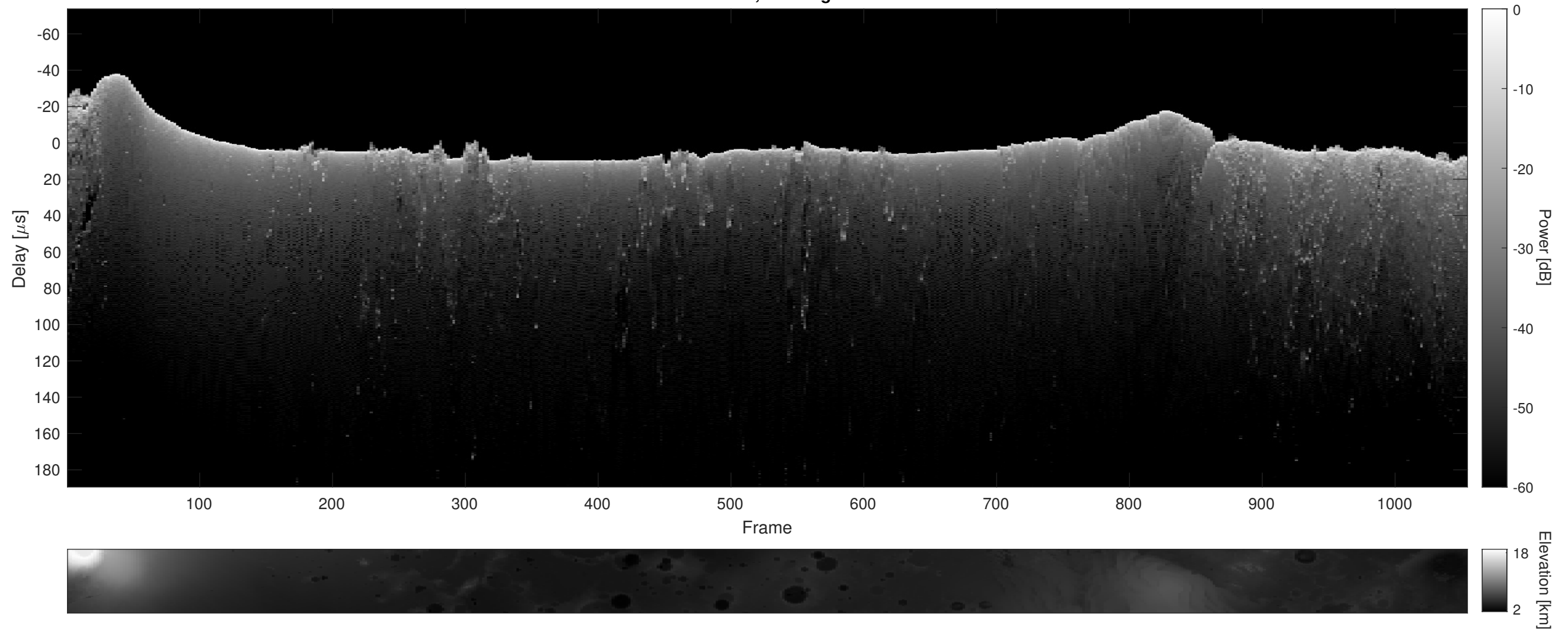
Orbit 2723, Cluttergram
