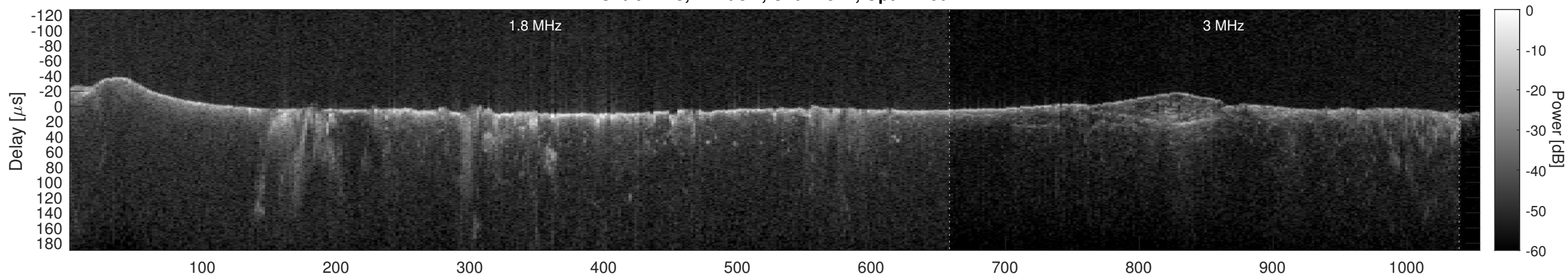
Orbit 2723, Cluttergram
