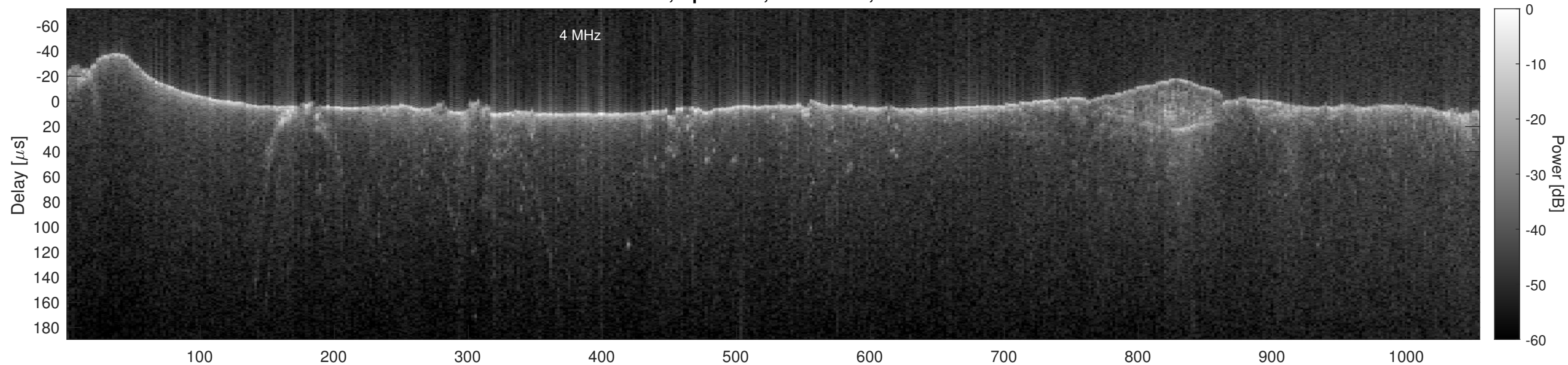
Orbit 2723, Optimized, No Window, Channel 2
