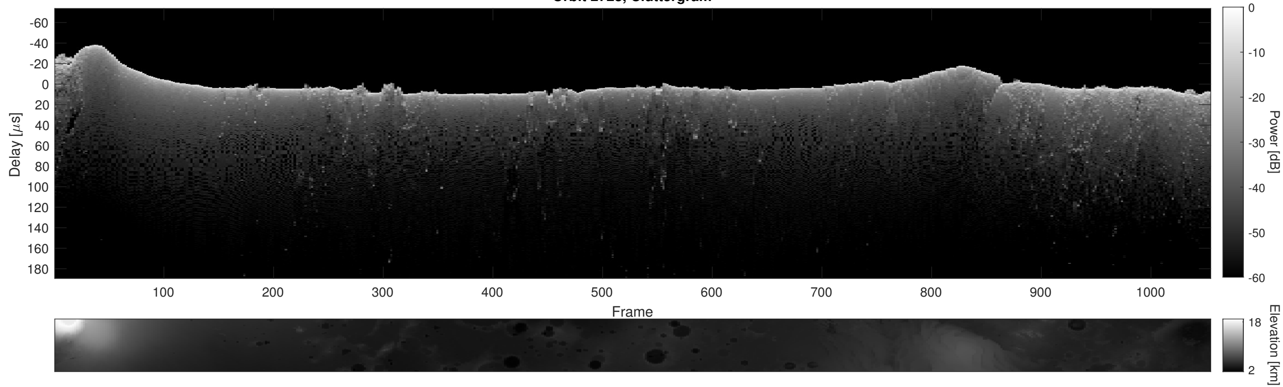
Orbit 2723, Cluttergram
