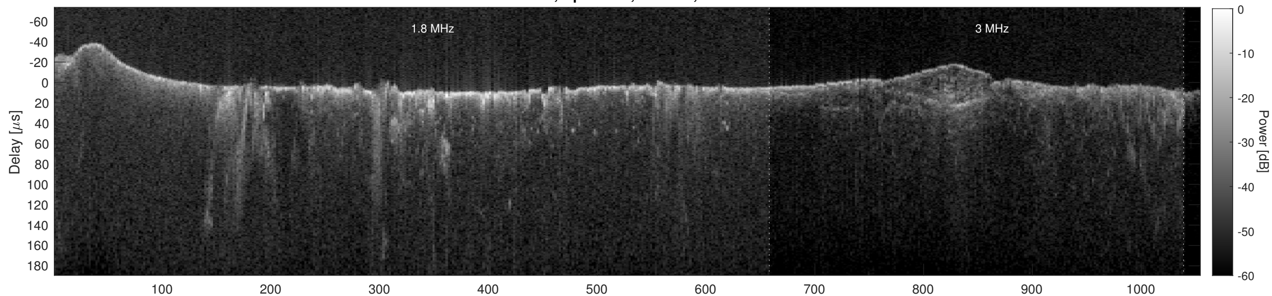
Orbit 2723, Cluttergram
