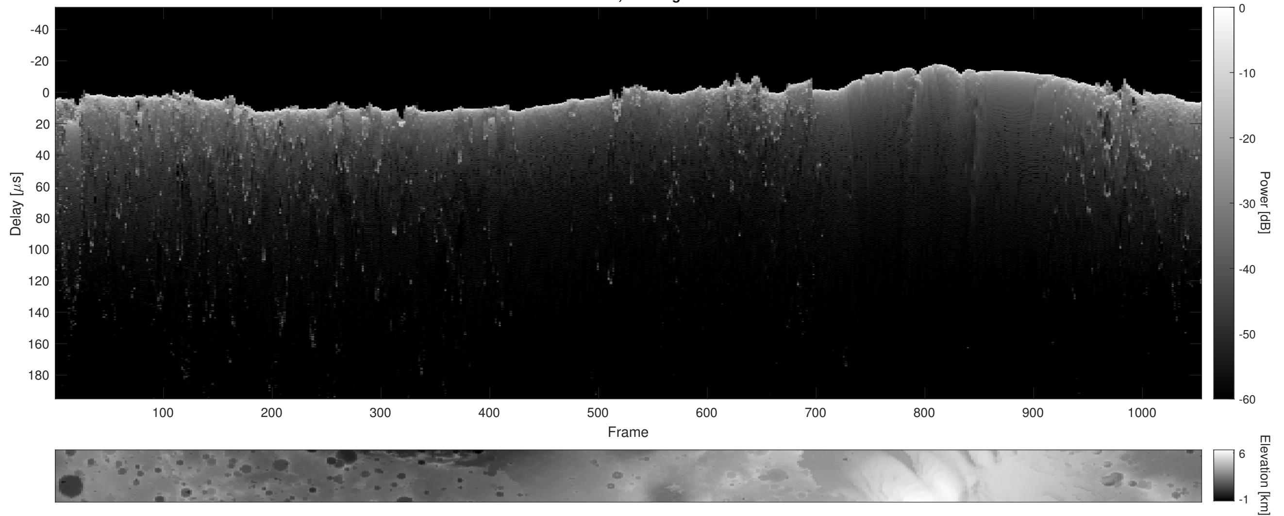
Orbit 2725, Cluttergram
