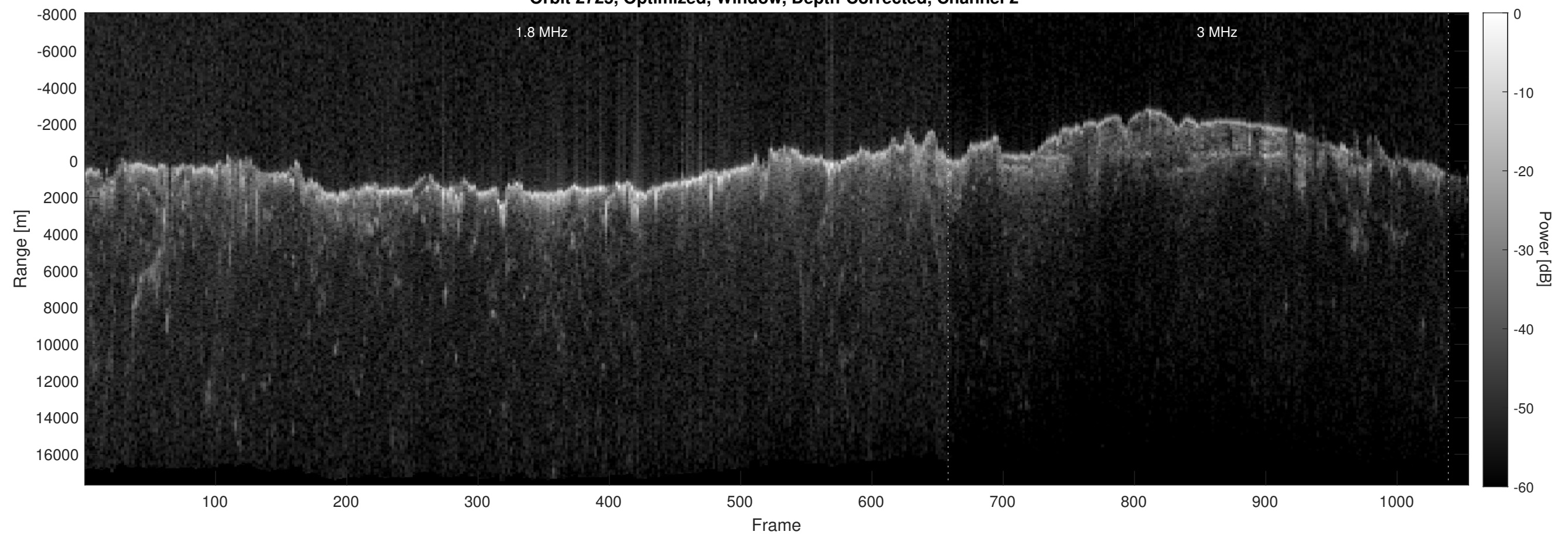
Orbit 2725, Optimized, Window, Depth-Corrected, Channel 2
