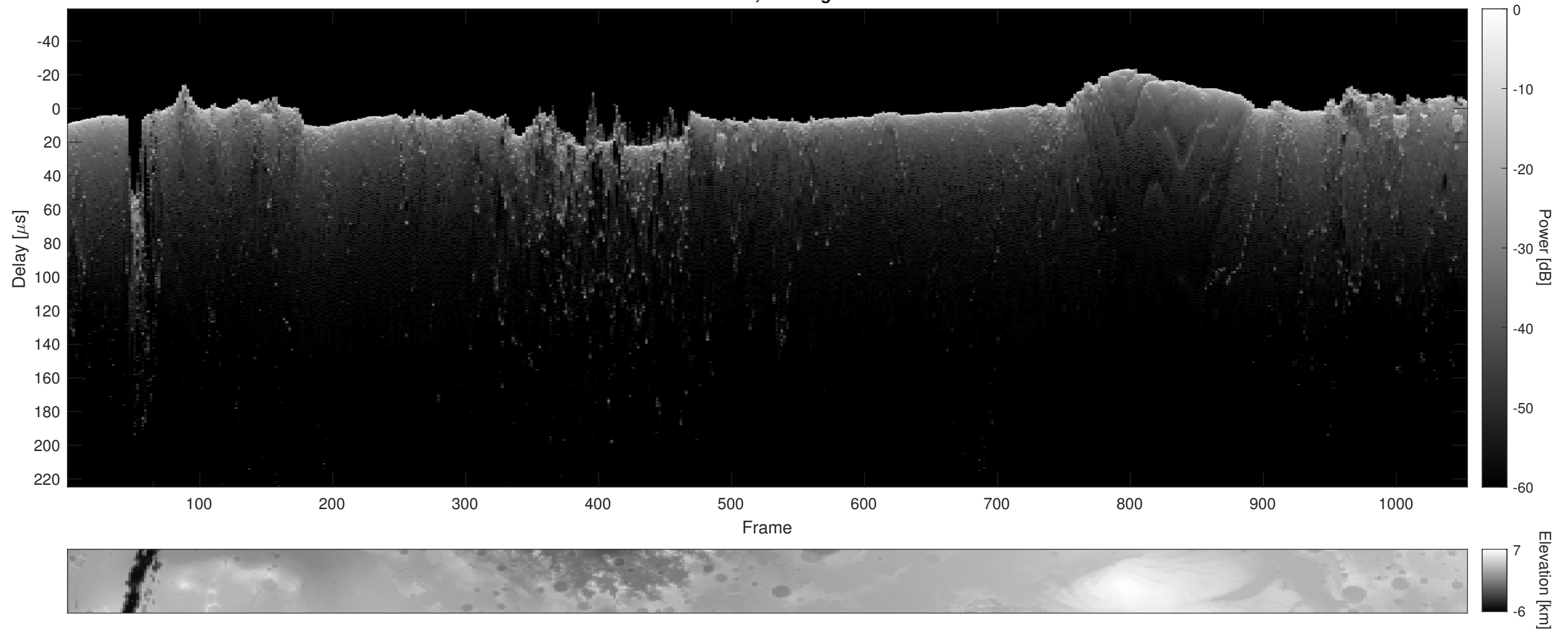
Orbit 2726, Cluttergram
