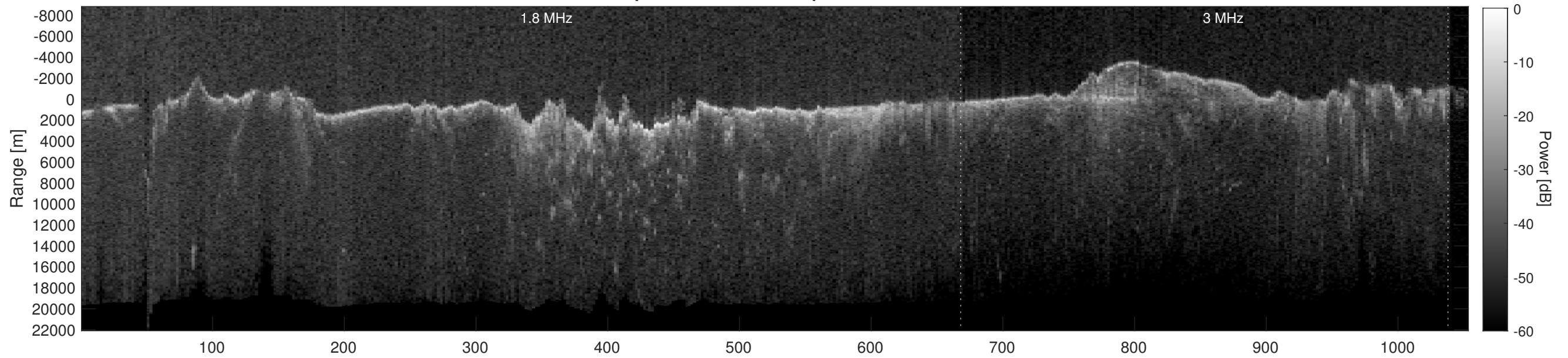
Orbit 2726, Depth-Corrected Cluttergram
